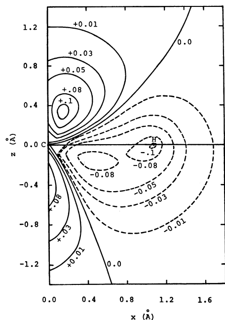
Figure 5. The change in the density distribution along the C_1-H_2 bond on the \pi plane induced by the twisting motion at \theta = 45^\circ for the configuration (\pi)^1(\pi^*)^1 .
