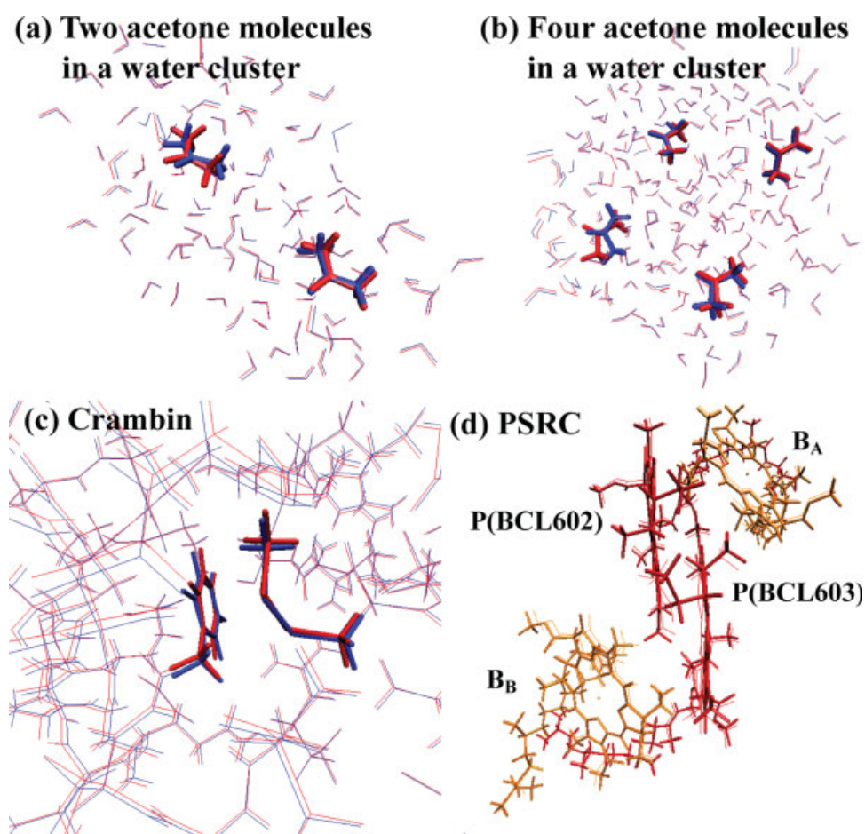
Figure 8. (a–c) Superposition of the structures optimized by the sc and mcQM/MM calculations. The structures shown in blue and red were obtained by the single-core and multicore approaches, respectively. (d) Superposition of the mcQM/MM (thick lines) and X-ray structures (thin lines) of the photosynthetic reaction center protein. Only P, B A , and B B are shown for the simplicity.
