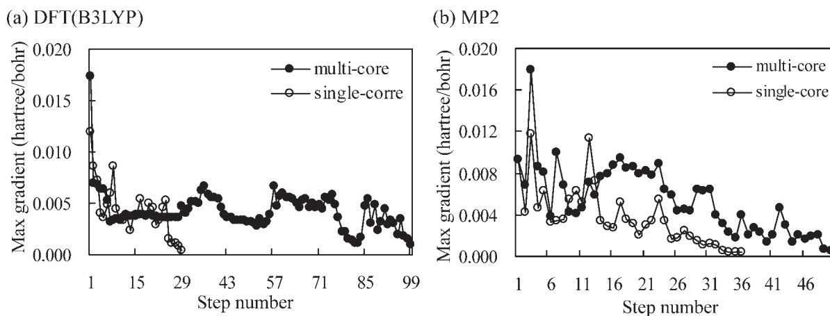
Figure 6. Maximum energy gradient (hartree/bohr) in each step of the optimization calculated by (a) DFT(B3LYP) and (b) MP2 methods. Calculations were performed for crambin in the ground state.
