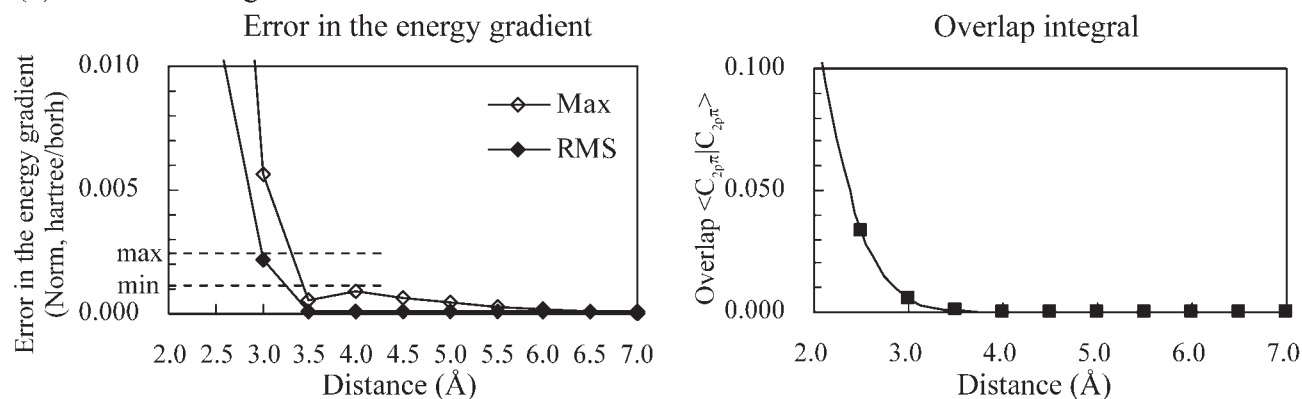
Figure 4. Intermolecule-distance dependence in the error of the energy gradient calculated by the multicore approach: (a) Two waters and (b) two benzene molecules in the ground states. Overlap integrals between the monomers are also compared.
