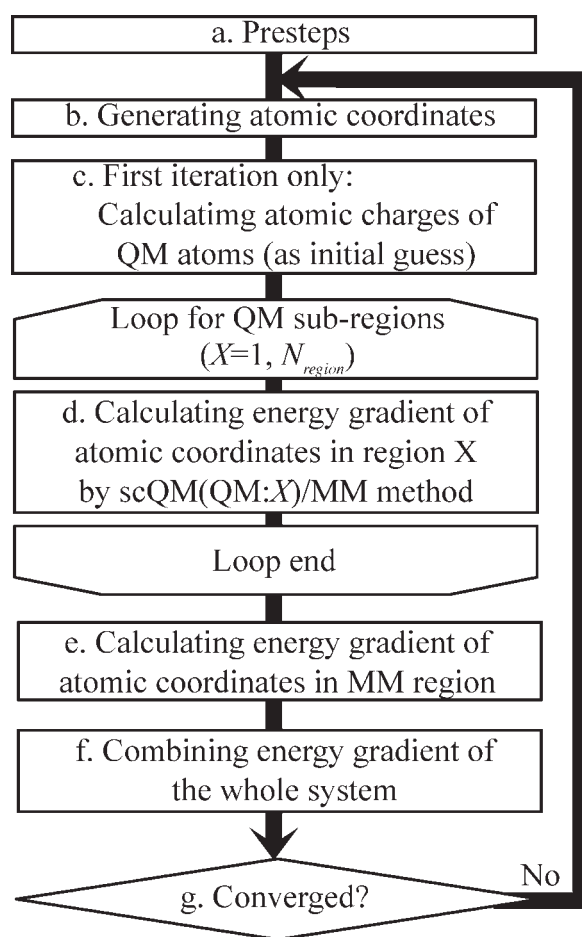
Figure 2. A flow chart of the mcQM/MM calculation for the geometry optimization.
