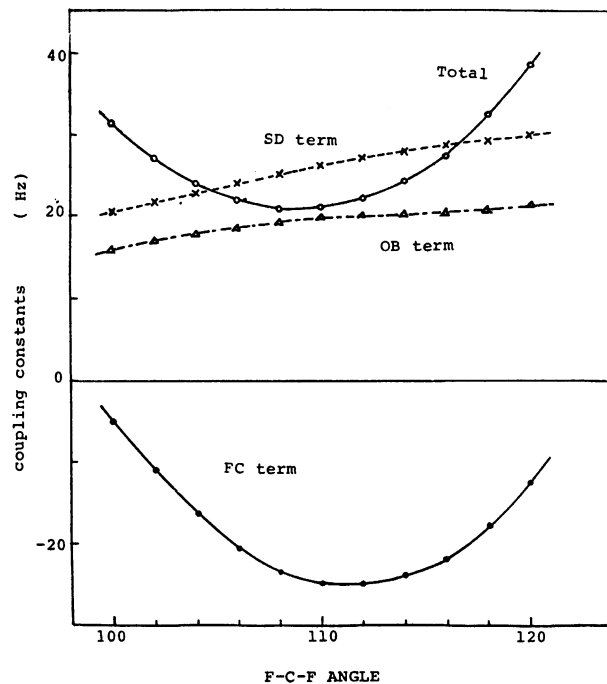
Figure 2. Plots of J_{FF}^{gem} vs. the FCF angle for CH_2=CF_2^* .
