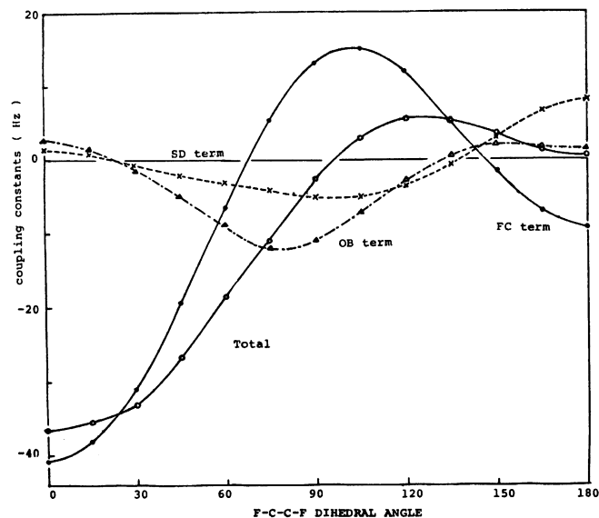
Figure 6. Plots of J_{FF}^{vic} vs. the FCCF dihedral angle, \theta , for \text{F}_2\text{CF}^*-\text{COF}^* .
