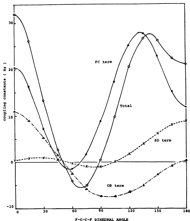
Figure 4. Plots of J_{FF}^{vic} vs. the FCCF dihedral angle, \theta , for \text{CH}_2\text{F}^*-\text{CH}_2\text{F}^* .
