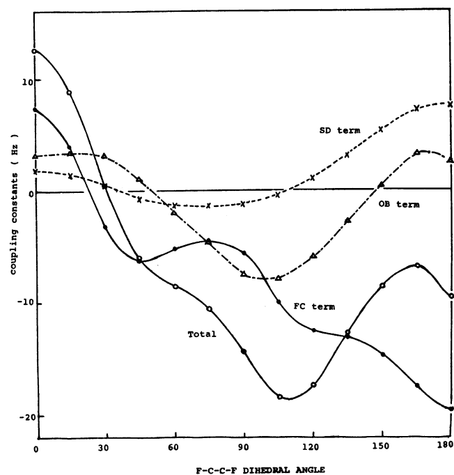
Figure 7. Plots of J_{FF}^{vic} vs. the FCCF dihedral angle, \theta , for \text{F}_2\text{CF}^*-\text{F}^*\text{C}=\text{CF}_2 .
