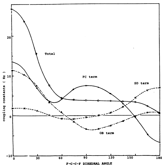
Figure 5. Plots of J_{FF}^{vic} vs. the FCCF dihedral angle, \theta , for \text{F}_2\text{CF}^*-\text{CH}_2\text{F}^* .
