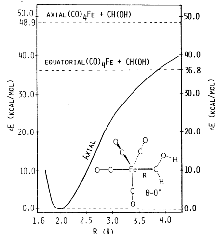
Figure 5. Potential curve for the singlet dissociation of the Fe=C carb bond of (CO) 4 Fe=CH(OH).
