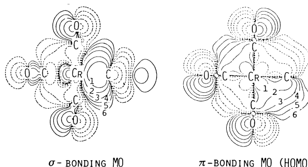
Figure 7. Contour maps of the \sigma and \pi bonding MO's of (\text{CO})_5\text{Cr}=\text{CH}(\text{OH}) . The intersection is perpendicular to the plane of the carbene group and includes the \text{Cr}-\text{C}_{\text{carb}} bond. Solid and broken lines correspond to the plus and minus signs in the MO's. The numbers 1-6 on contours correspond to the values (au) 0.1, 0.05, 0.02, 0.01, 0.005, 0.002, respectively.
