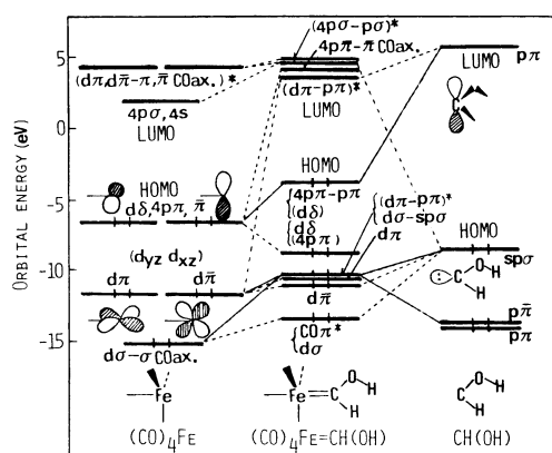
Figure 9. Correlation diagram of orbitals of the axial (\text{CO})_4\text{Fe}=\text{CH}(\text{OH}) with those of the axial (\text{CO})_4\text{Fe} and \text{CH}(\text{OH}) in the singlet state. ( \bar{\pi} denotes an AO perpendicular to the \pi AO).
