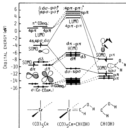
Figure 8. Correlation diagram of orbitals of (\text{CO})_5\text{Cr}=\text{CH}(\text{OH}) with those of the triplet fragments ( \bar{\pi} denotes an AO perpendicular to the \pi AO).
