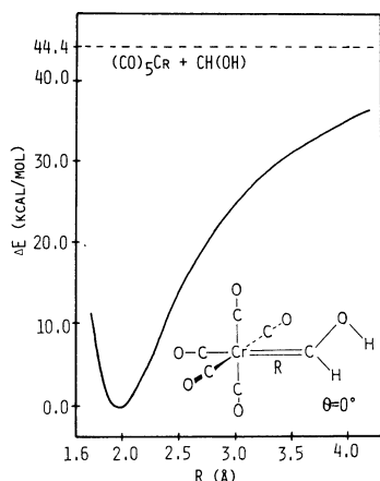
Figure 4. Potential curve for the singlet dissociation of the Cr=C carb bond of (CO) 5 Cr=CH(OH).
