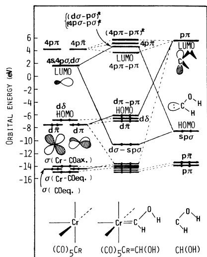
Figure 6. Correlation diagram of orbitals of (\text{CO})_5\text{Cr}=\text{CH}(\text{OH}) with those of the singlet fragments ( \bar{\pi} denotes an AO perpendicular to the \pi AO).
