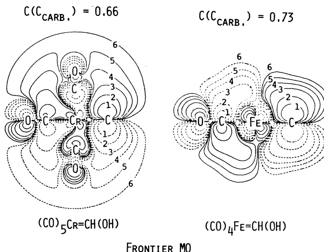
Figure 12. Contour maps of the LUMO's of (CO) 5 Cr=CH(OH) and axial (CO) 4 Fe=CH(OH). The intersection is perpendicular to the plane of the carbene group and includes the M-C carb bond. Solid and broken lines correspond to the plus and minus signs in the MO's. The numbers 1-6 on contours correspond to the values (au) 0.1, 0.05, 0.02, 0.01, 0.005, 0.002, respectively. C(C carb ) denotes the coefficient of the p\pi AO of the carbene carbon atom in the LUMO.
