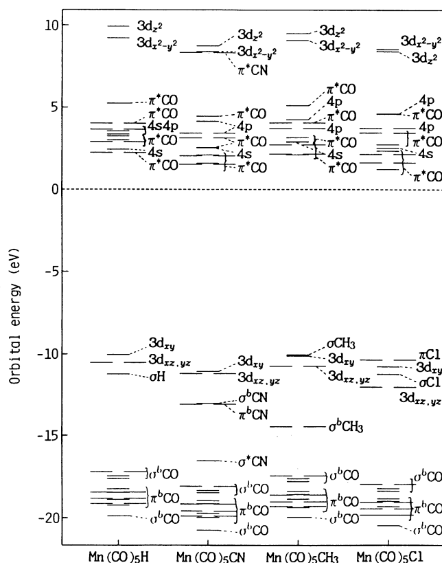
Figure 3. Orbital energy diagrams for the manganese complexes, Mn(CO) 5 L (L = H, CN, CH 3 , Cl) (3d z 2 = 3d σ , 3d xz, yz = 3d π , 3d xy = 3d δ1 , 3d x 2 -y 2 = 3d δ2 ).
