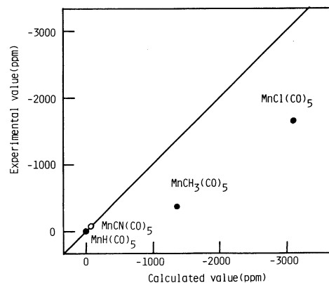
Figure 1. Comparison between experimental and calculated values for ^{55}\text{Mn} magnetic shielding constants in manganese complexes. For the \text{Mn}(\text{CO})_5\text{CN} complex, no experimental data have been reported, so the open circle shows only the calculated value.
