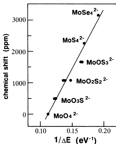
Figure 1. Relationship between the inverse of the lowest magnetically allowed d-d* excitation energies \Delta E and the chemical shifts. The chemical shifts are the experimental values due to Gheller et al. 14 and the excitation energies are the SAC-CI theoretical values for the 4d\sigma \rightarrow 4d\pi^* transitions with the T_1 ( T_d ), A_2 + E ( C_{3v} ), and A_2 + B_1 + B_2 ( C_{2v} ) symmetries. The correlation factor is 0.987 in the least-squares fitting. 18
