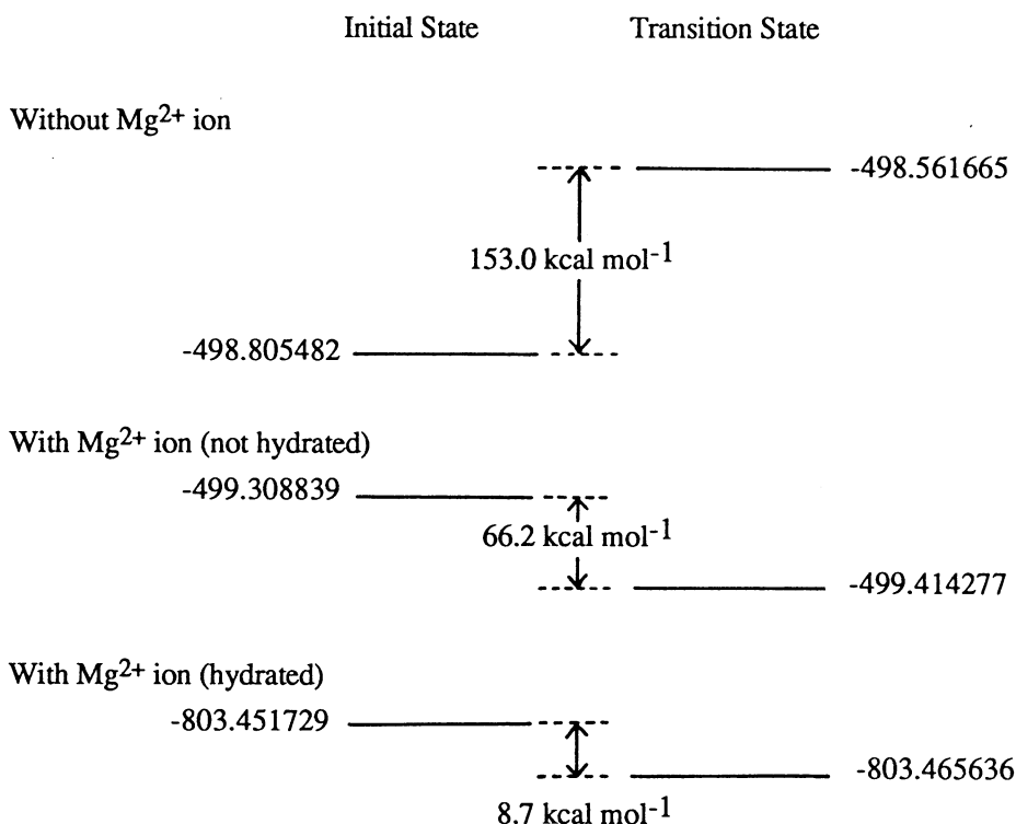
Fig. 3. Energy profile of the initial and transition states of the reaction with or without Mg 2+ ion.
