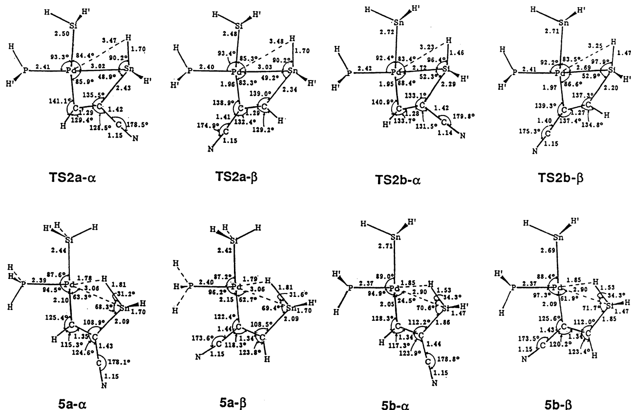
Figure 16. Optimized structures of the transition states and products 5 inserted in cyanoacetylene. TS2x-y and 5x-y ( x = a, b ; y = \alpha, \beta ) are defined in Figure 3. H'' indicates the two hydrogens above and below the plane.
