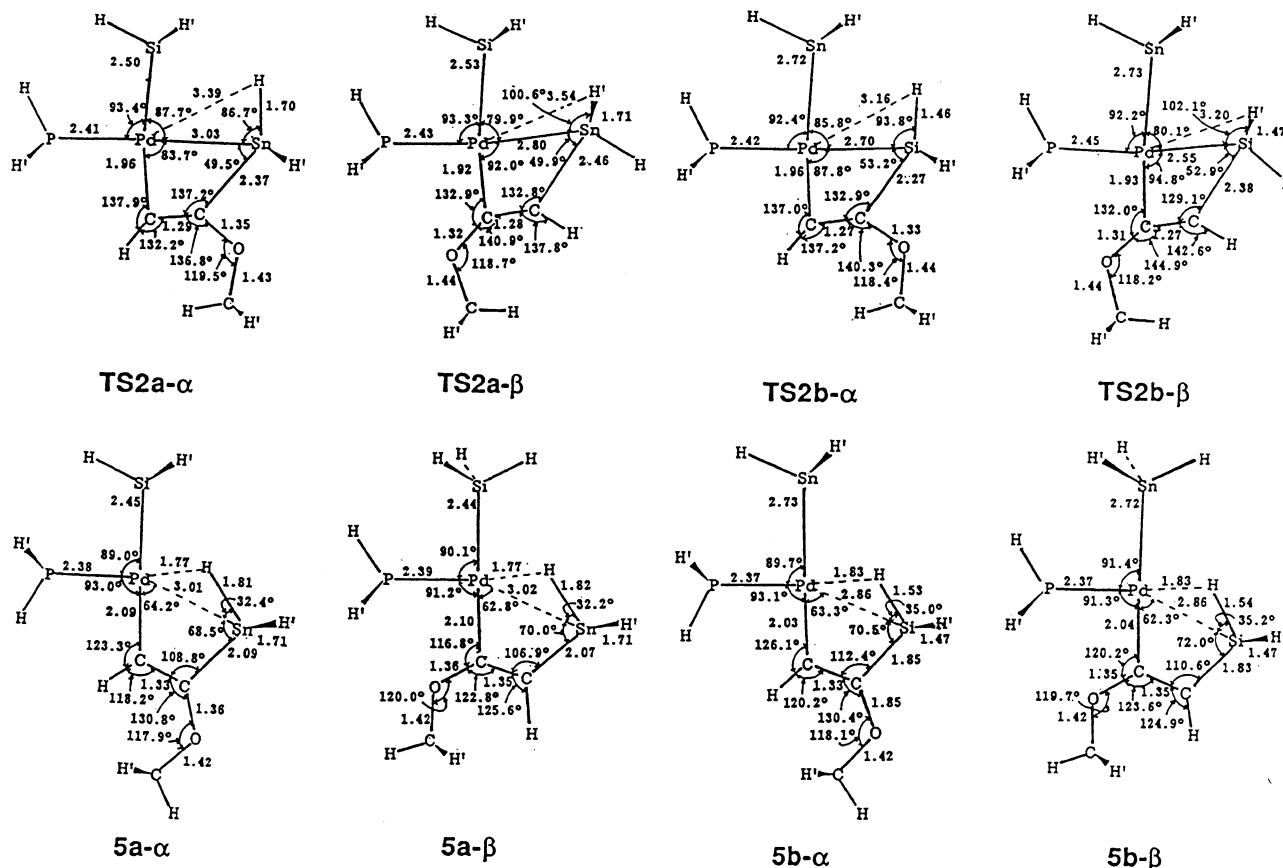
Figure 15. Optimized structures of the transition states and products 5 inserted in methoxyacetylene. TS2x-y and 5x-y ( x = a, b; y = \alpha, \beta ) are defined in Figure 3. H' indicates the two hydrogens above and below the plane.
