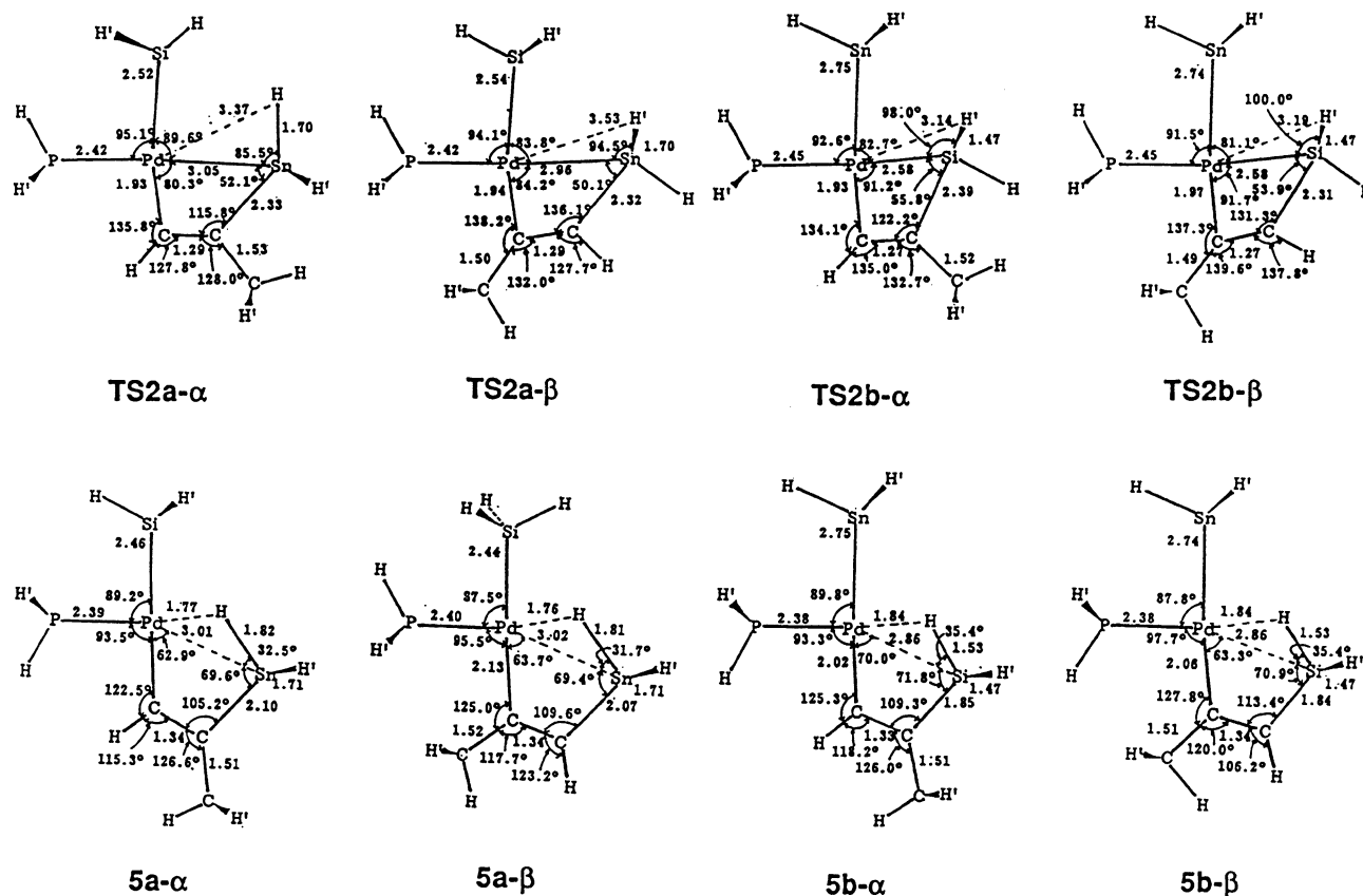
Figure 14. Optimized structures of the transition states and products 5 inserted in methylacetylene. TS2x-y and 5x-y (x = a, b; y = \alpha , \beta ) are defined in Figure 3. H' indicates the two hydrogens above and below the plane.
