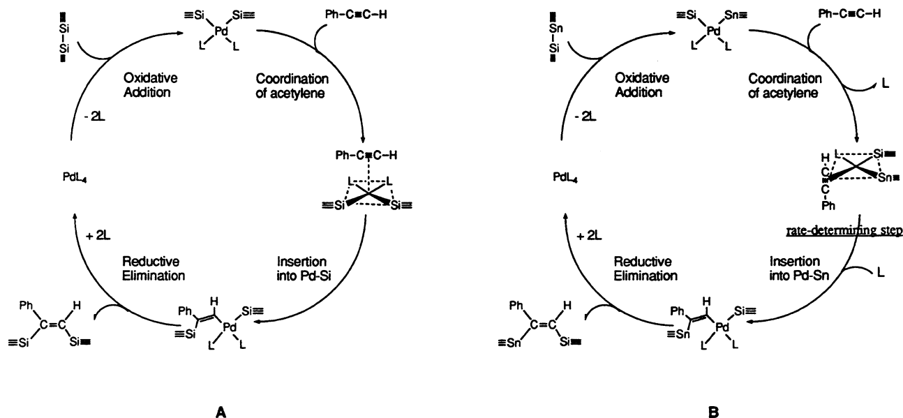
Figure 1. Reaction scheme (A) suggested by Nagai et al. 24 for bis-silylation and (B) adopted in this paper for silastannation.
