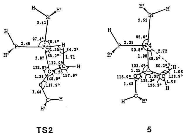
Figure 12. Structures of the transition state and the inserted product 5 in hydrosilylation (R = OCH 3 ). H' indicates the two hydrogens above and below the plane.
