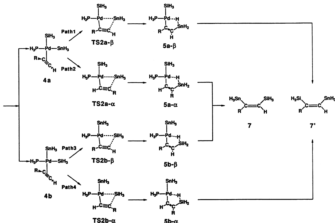
Figure 3. Possible reaction schemes for the insertion step. Acetylenes substituted by R insert into the Pd–Sn bond (top) or the Pd–Si bond (bottom). The \alpha and \beta indicate at which carbon the addition of Si or Sn occurs.
