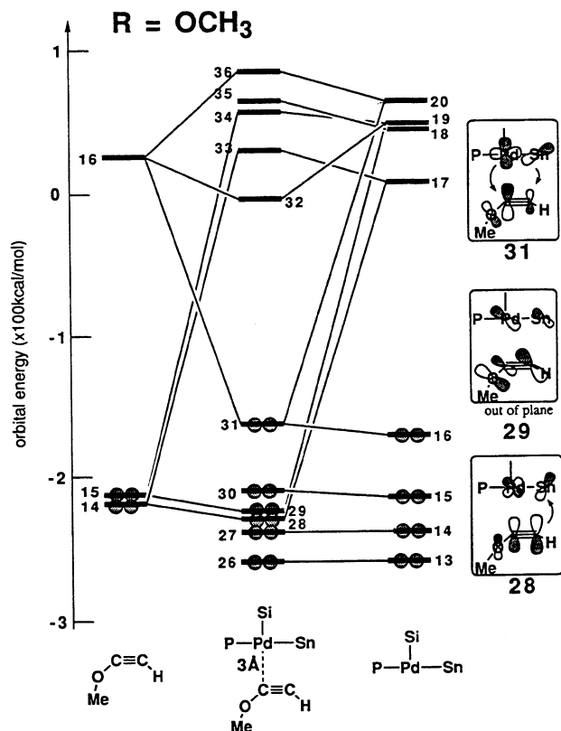
Figure 6. Orbital correlation diagram before TS2 when methoxyacetylene interacts with the palladium complex. They are separated by 3 Å, keeping the geometries in the transition state. The acetylene donates an electron to the palladium complex through the 28th orbital, and the palladium complex back-donates an electron to the acetylene through the 31st orbital.
