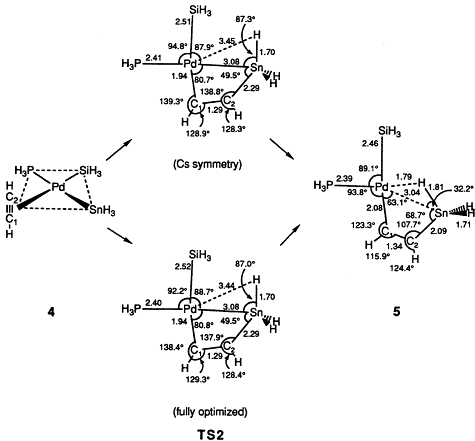
Figure 13. Schematic pictures and the optimized geometries of adducts 4 and 5 and the transition state TS2 (R = H). It is assumed that acetylene inserts into the Pd–Sn bond in TS2. The geometry for TS2 is optimized fully, keeping the C_s symmetry for comparison. The activation energies in this step are 24.1 kcal/mol (fully optimized) and 24.7 kcal/mol ( C_s ).
