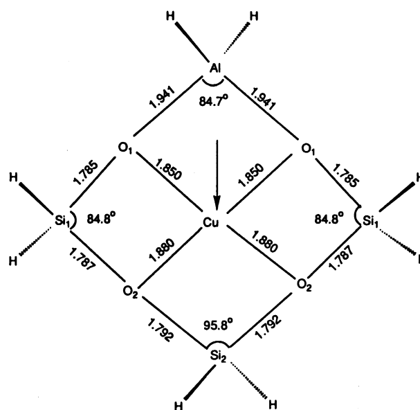
Fig. 1. Cluster model applied to the study of adsorption of CO and NO molecules on the Cu-containing active site of the four-membered ring of the zeolite catalyst. Subscript numbers label the distinct atomic centers. Optimized bond lengths and bond angles for H_8Si_3AlO_4Cu^+ are in angstroms and degrees, respectively. The arrow indicates the adsorption place for CO and NO.
